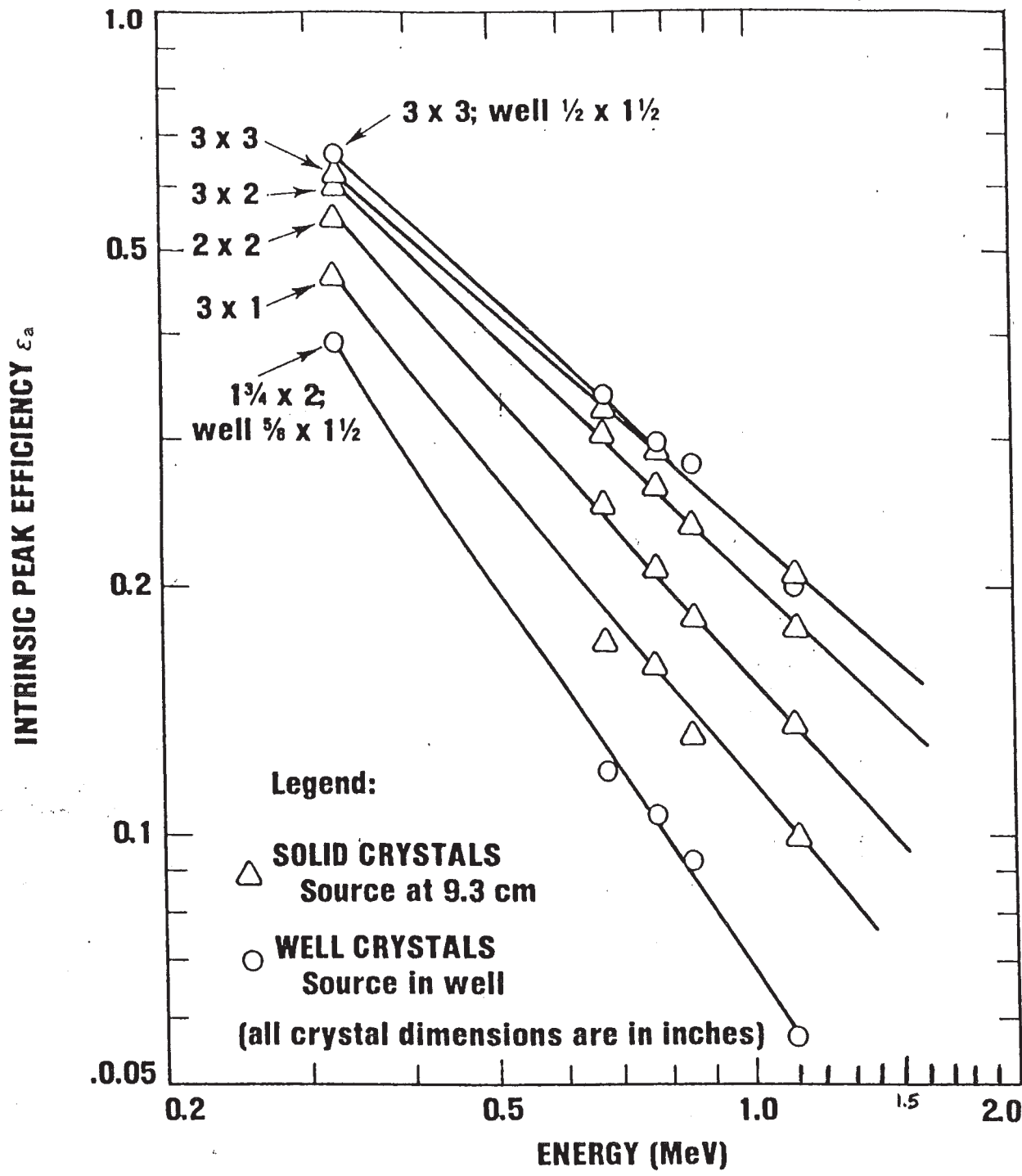
Figure 2.14. Intrinsic peak efficiency ( \epsilon_a ) for a wide variety of NaI(Tl) crystals. The source to detector distance is 9.3 cm (Courtesy of Idaho Operations Office DOE).
