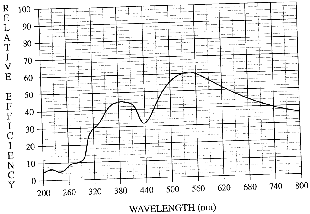
GRATING EFFICIENCY CURVE, MODEL 03 (1800 g/mm HOLOGRAPHIC GRATING, OPTIMIZED FOR THE VISIBLE)
