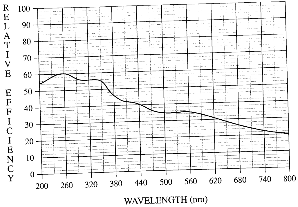
GRATING EFFICIENCY CURVE, MODEL 02 (1800 g/mm HOLOGRAPHIC GRATING, OPTIMIZED FOR THE U.V.)
